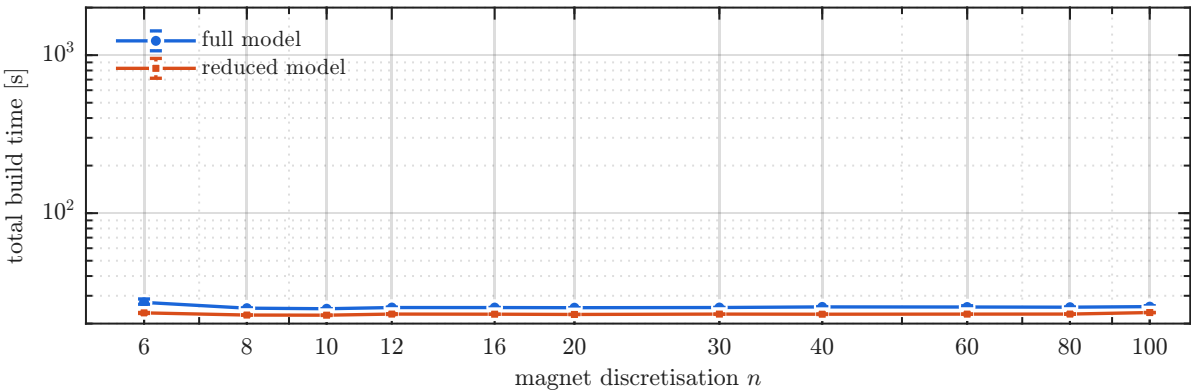
Iteration 3: mapped field, -O1 compile
